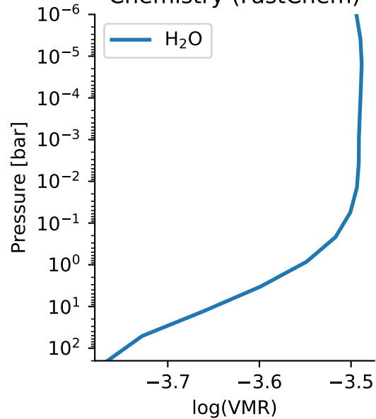
Chemistry (FastChem)
