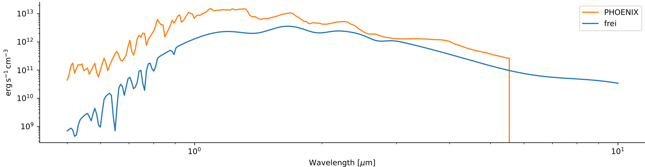
Emission spectrum
